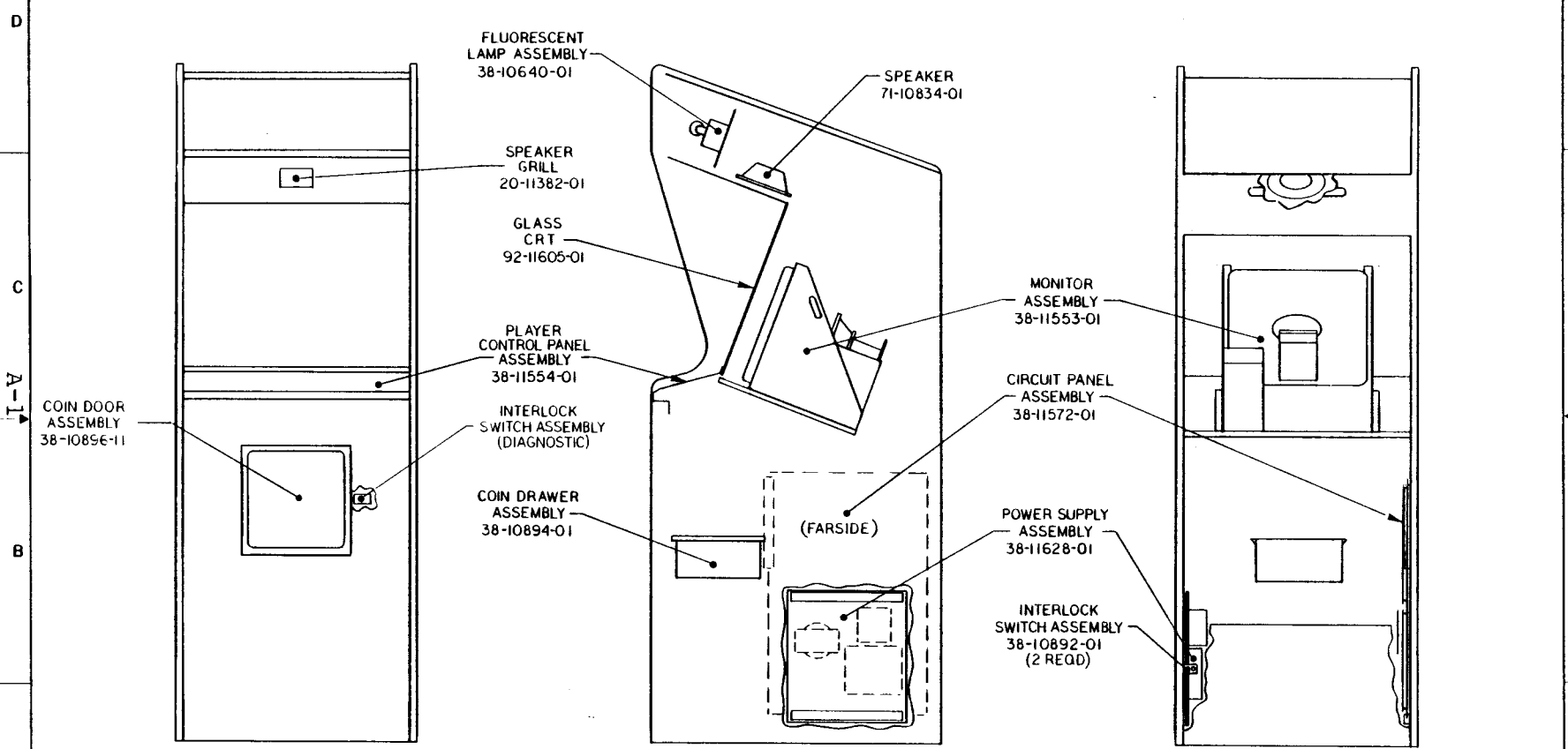
FRONT VIEW
